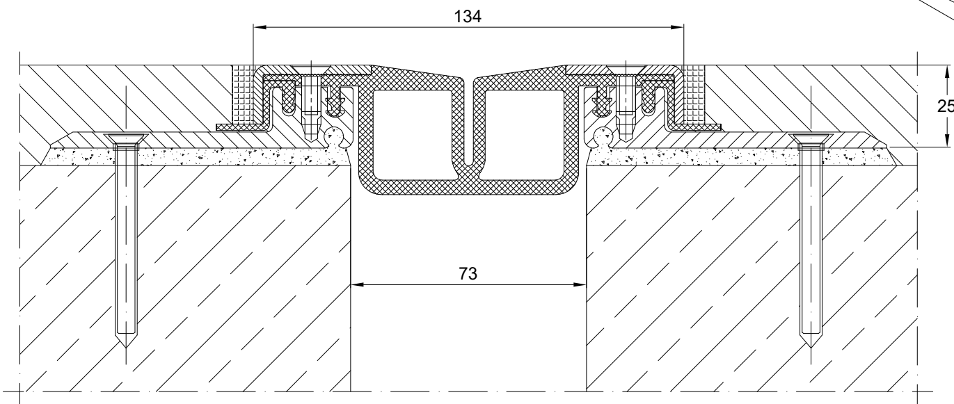
CONECTO GA 88.45.25 S SECTION
