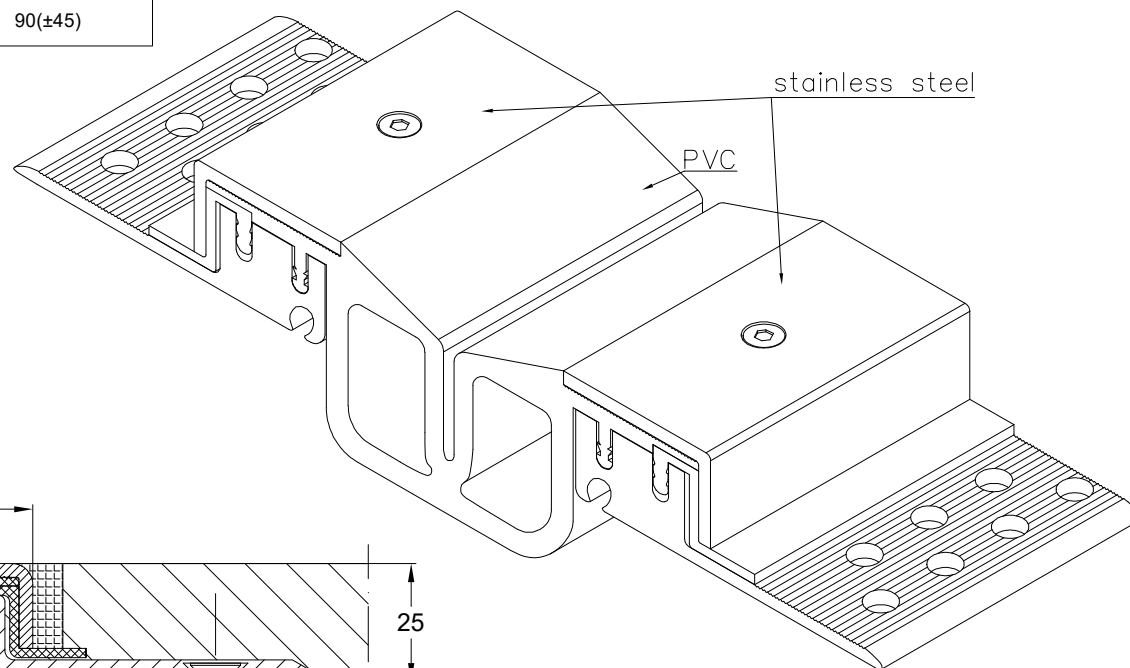
CONECTO GA 88.45.25 S VIEW
